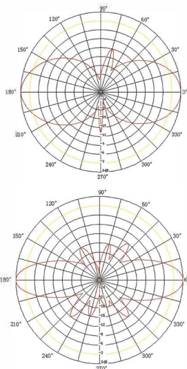
Horizontal Pattern (698-960/1710-2170)
